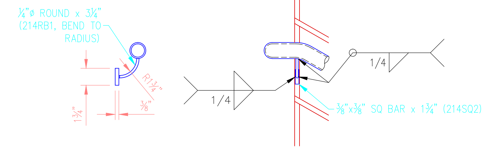
(C) HANDRAIL BRACKET BRACKET FOR LH POST IS SHOWN; BRACKETS FOR OTHER POSTS ARE SIMILAR
