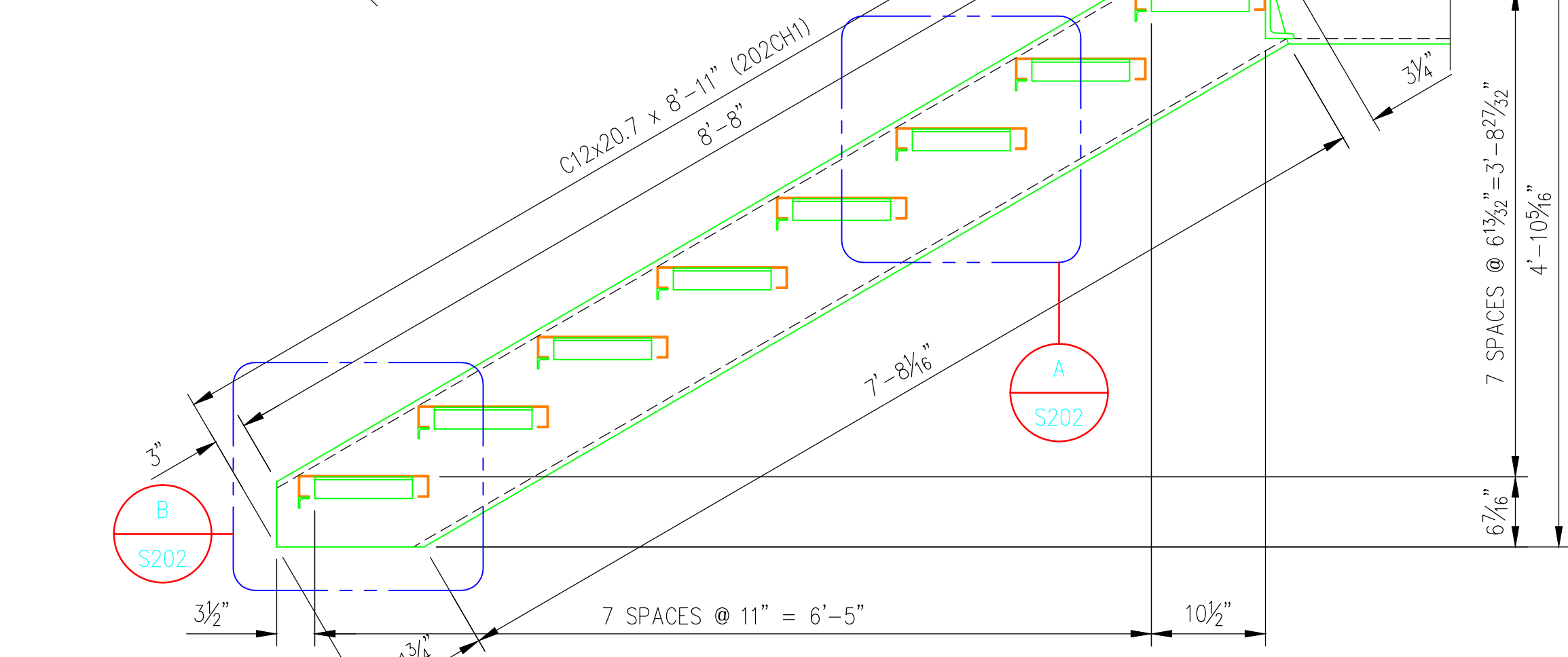
STAIR STRINGER 202CH1
