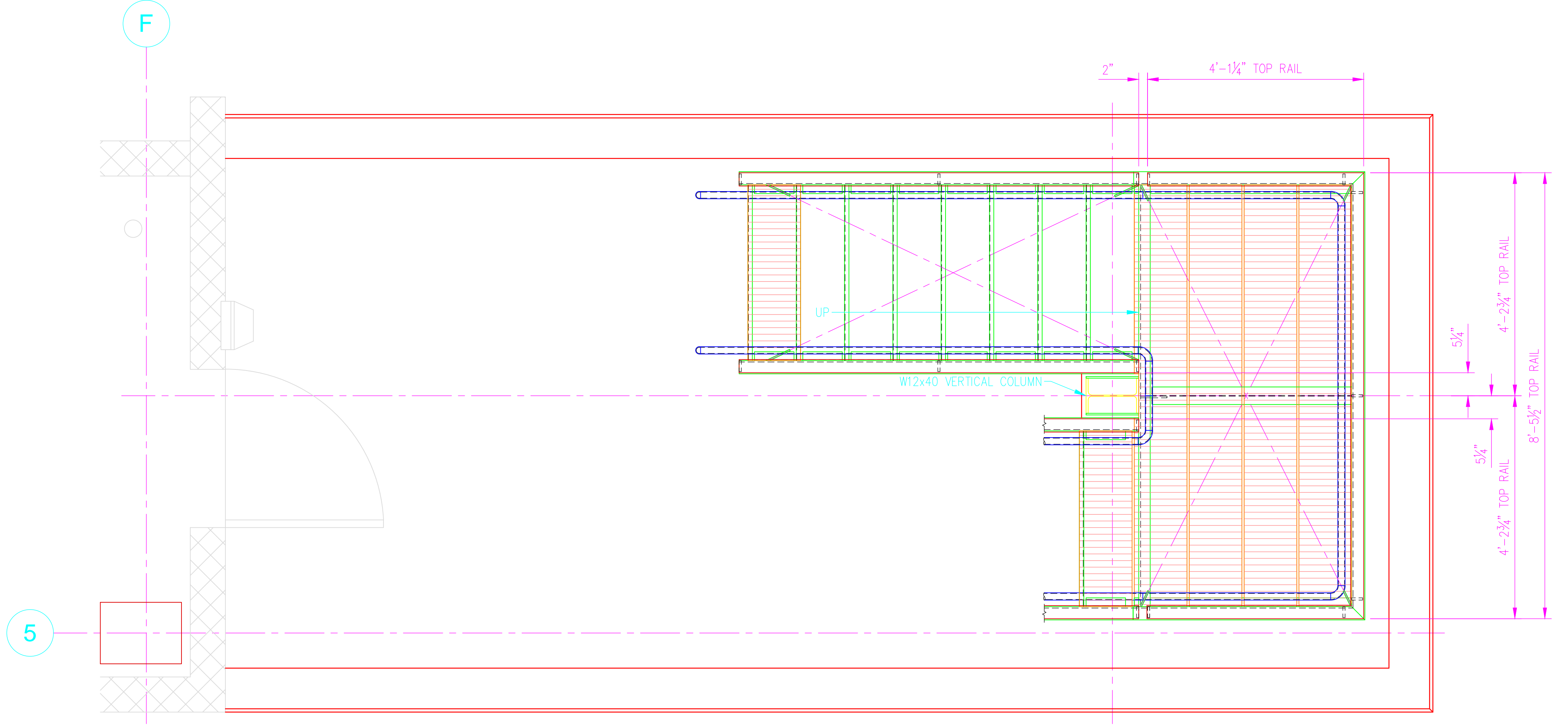
STAIR GUARDS AND HANDRAILS PLAN-LEVEL 1
