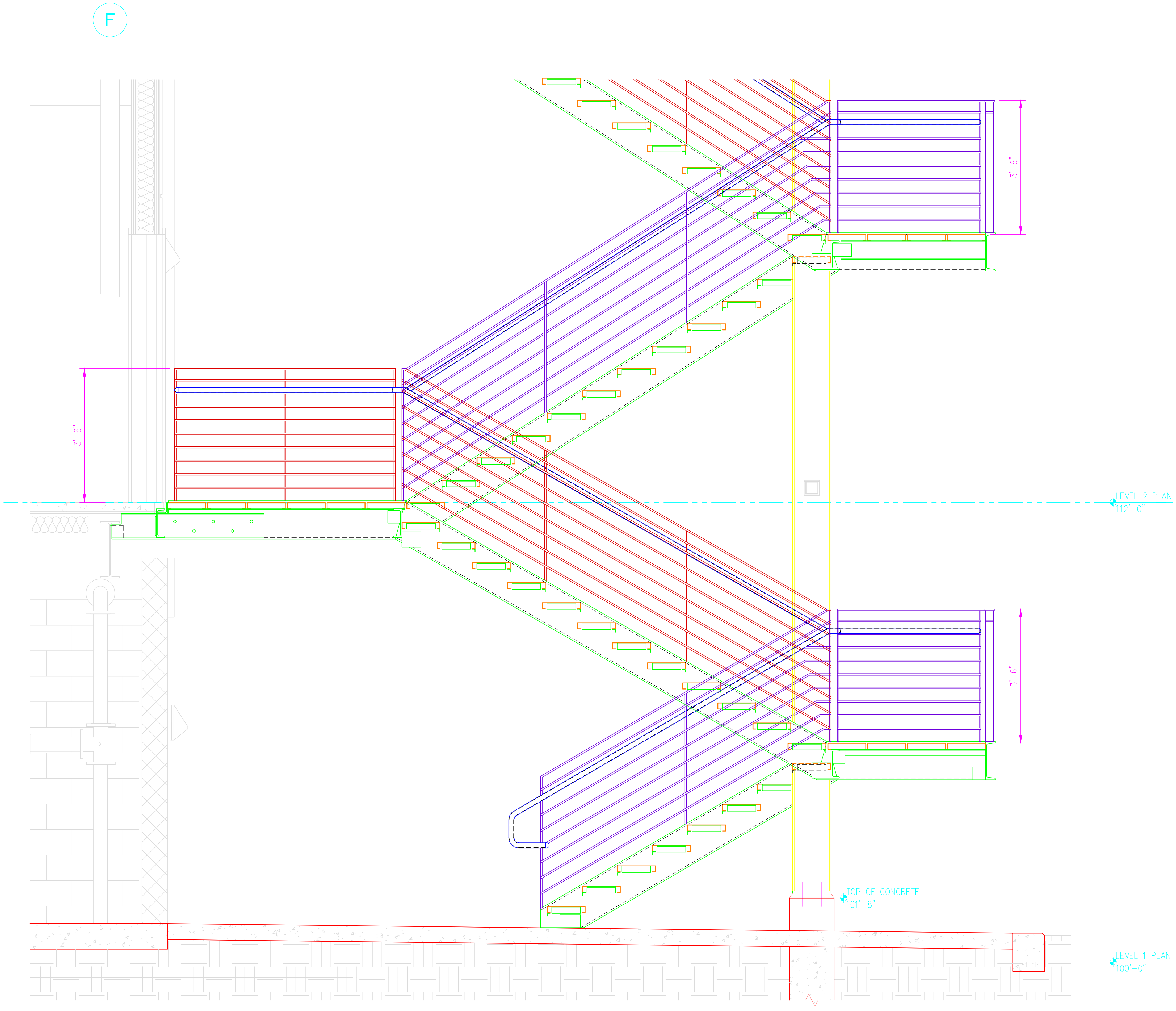
STAIRGUARDS AND HANDRAILS ELEVATION—LEVELS 1 & 2
