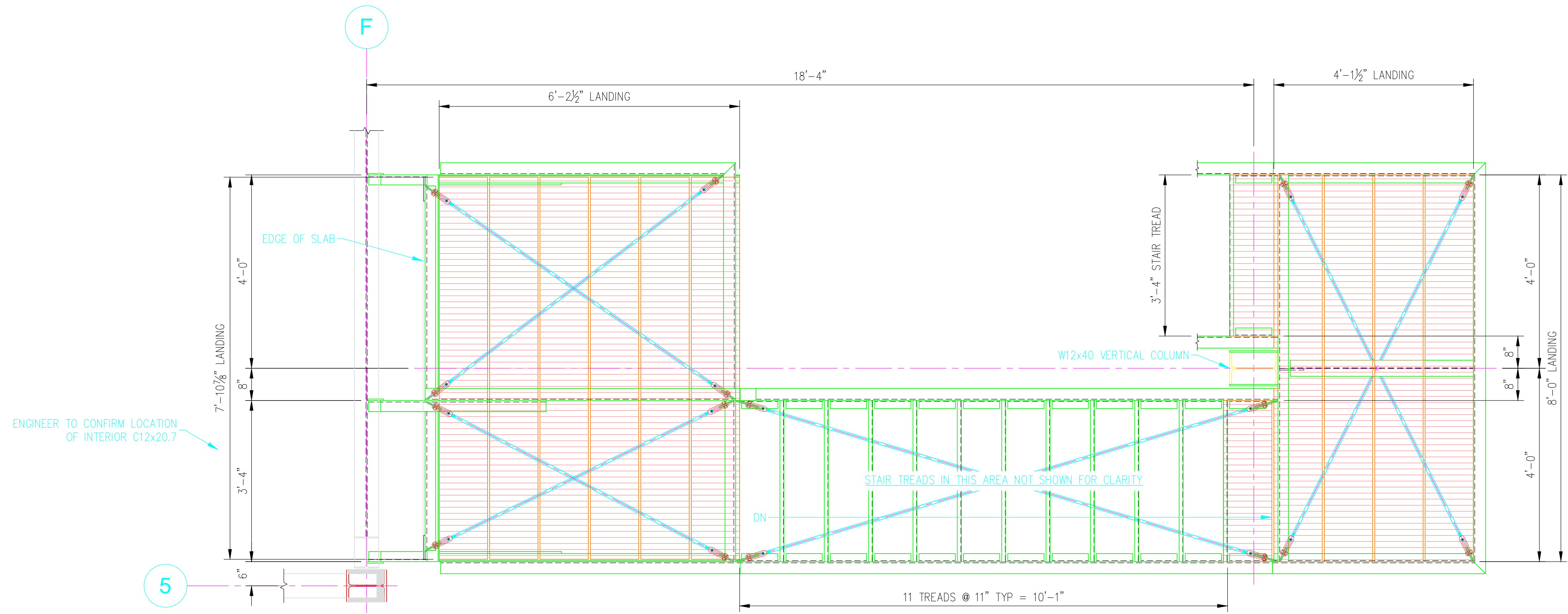
EXTERIOR STAIRS/STAIR 2 PLAN LEVEL 4
