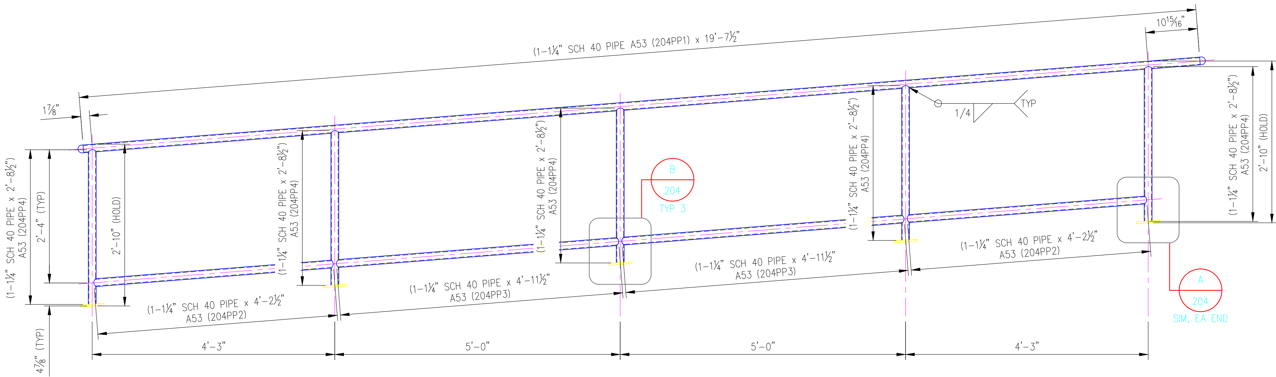
ELEVATION (FAR SIDE)
