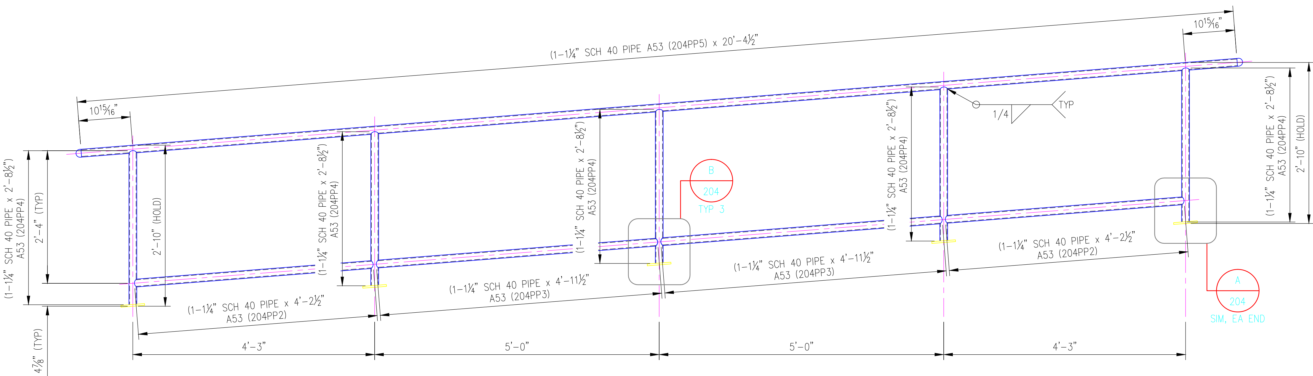
ELEVATION (NEAR SIDE)
