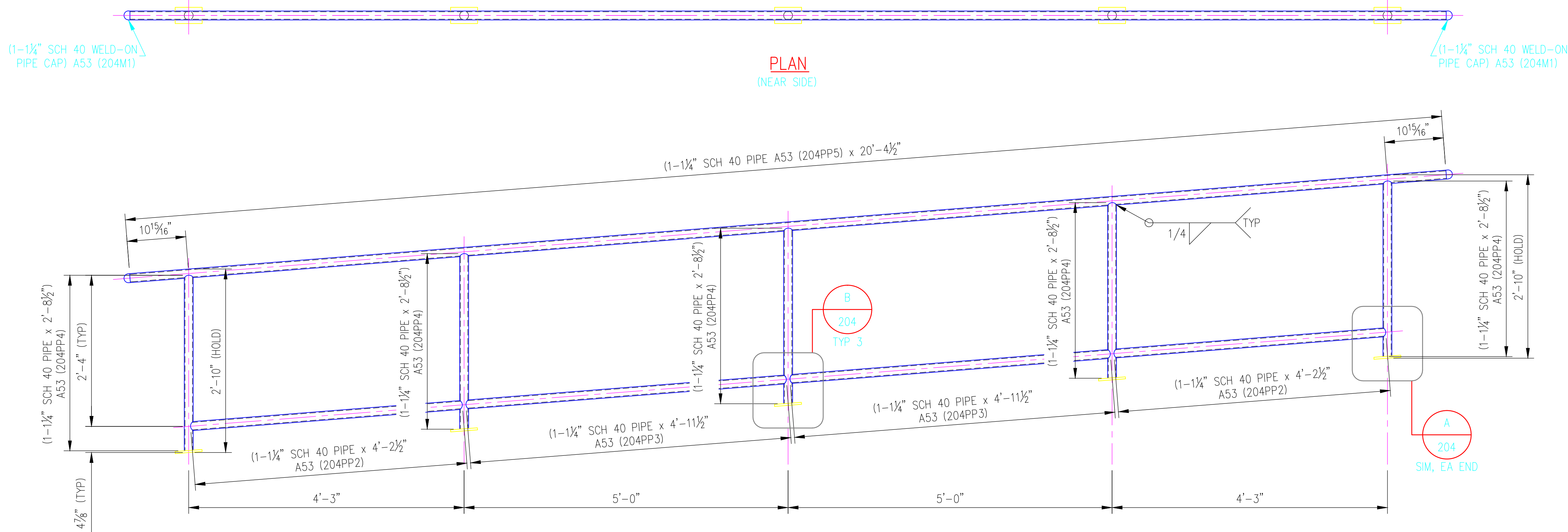
ELEVATION (NEAR SIDE)
