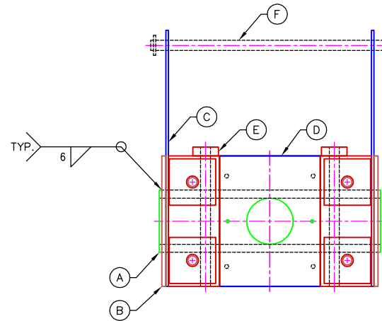
ELEVATION OF ASSEMBLED SATELLITE ANCHOR--(2 REQ'D) (SEE DRAWING 2207/225 FOR PARTS A,B,C,D,E & F) (SHOWN 2X ACTUAL SCALE)
