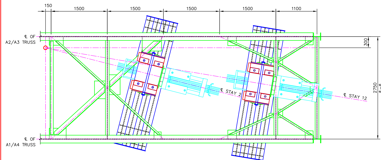
LOWER PLAN VIEW
