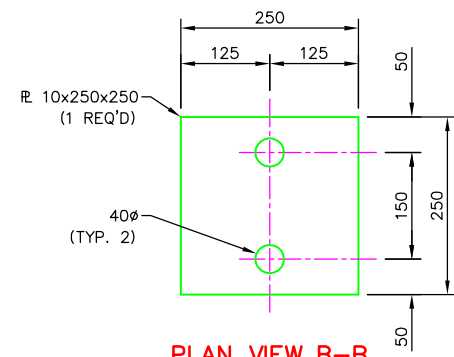
PLAN VIEW B-B
