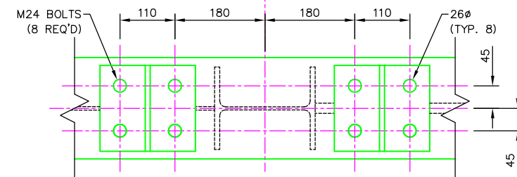
PLAN VIEW D-D BOLT LAYOUT ON TOP CHORD
