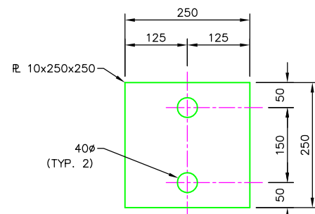
PLATE SPACER (4 REQ'D)
