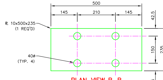
PLAN VIEW B-B
