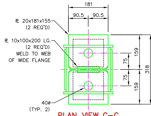
PLAN VIEW C-C
