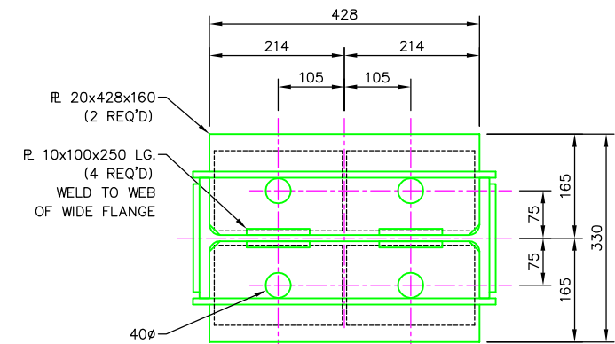
PLAN VIEW C-C
