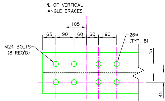
PLAN VIEW D-D BOLT LAYOUT ON TOP CHORD
