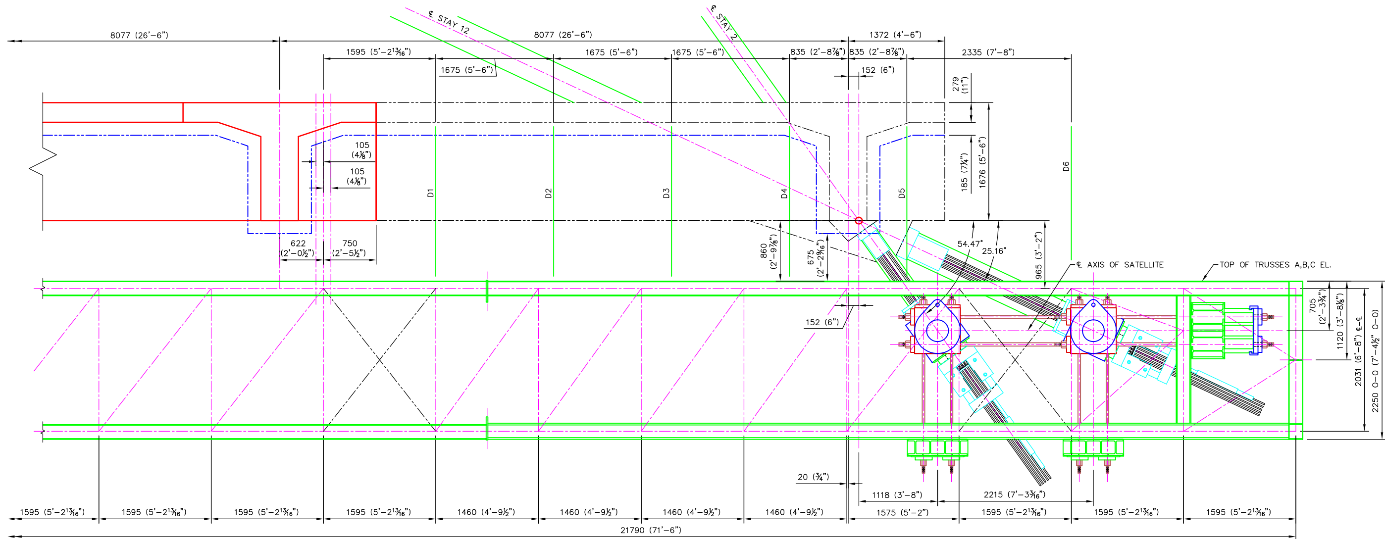
TRUSS A1/A4 ELEVATION
