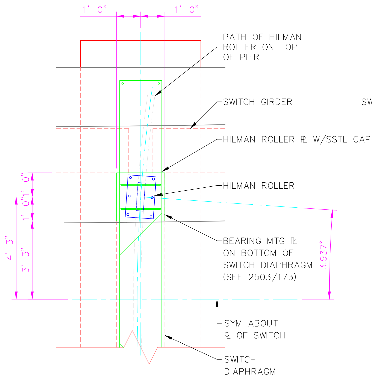
BEARING MOUNTING R. LOCATION PIER NO 4
