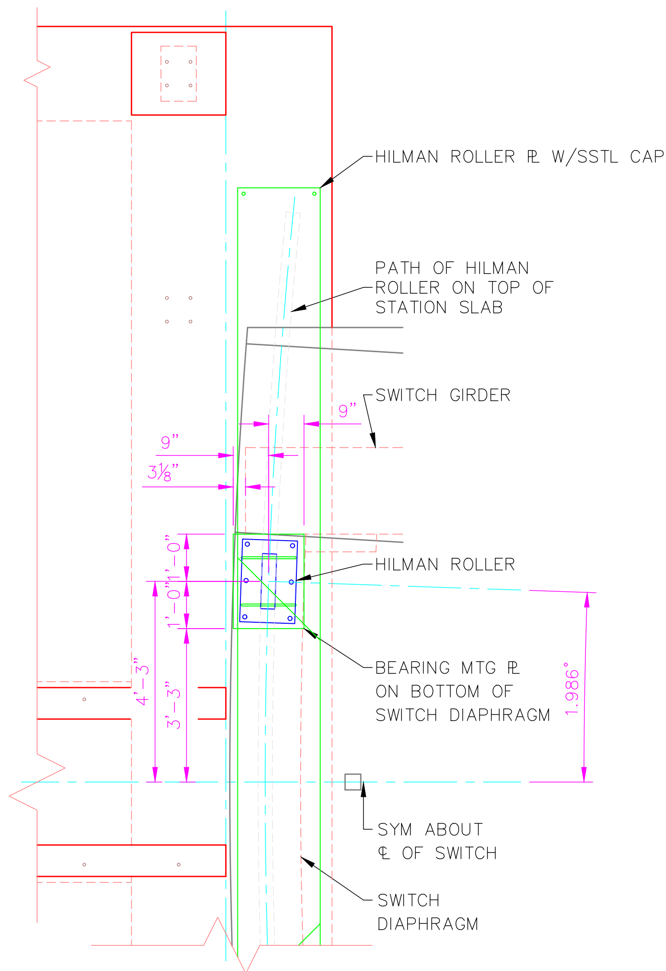
BEARING MOUNTING R. LOCATION PIER NO 3
