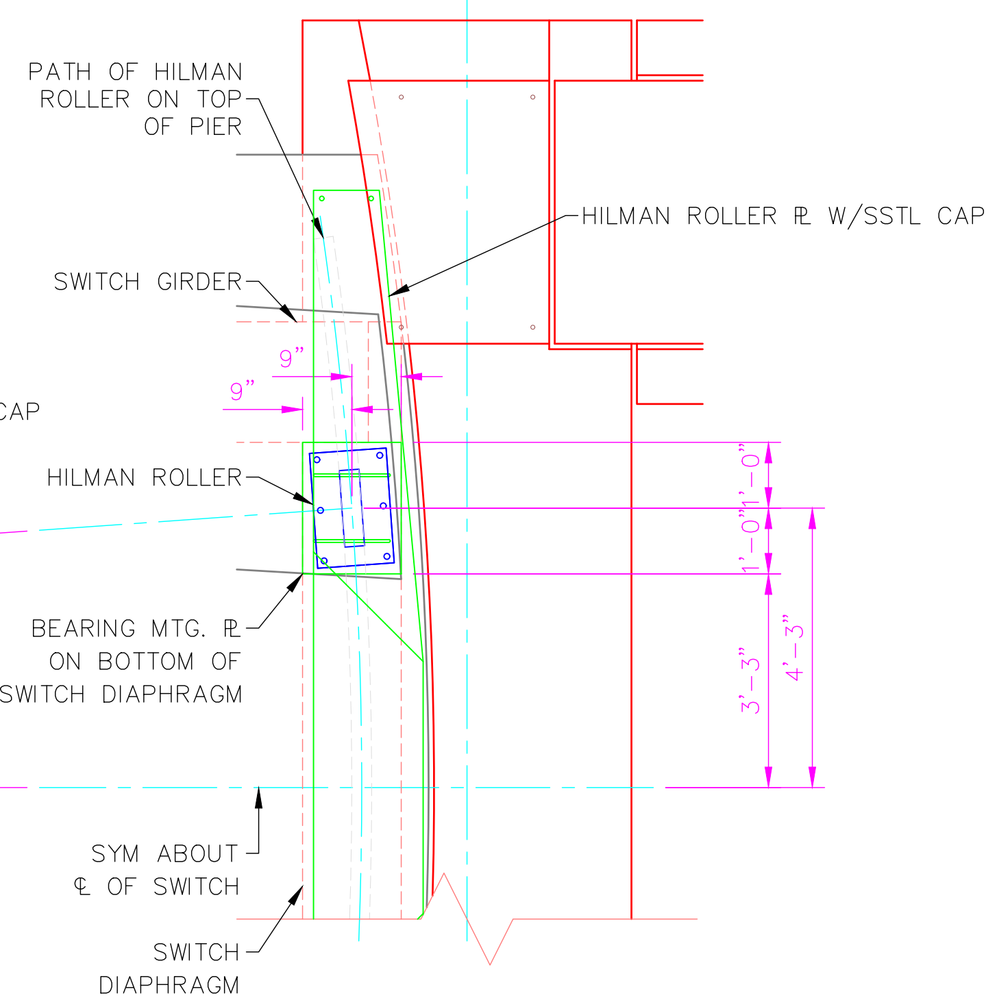
BEARING MOUNTING R. LOCATION PIER NO 6
