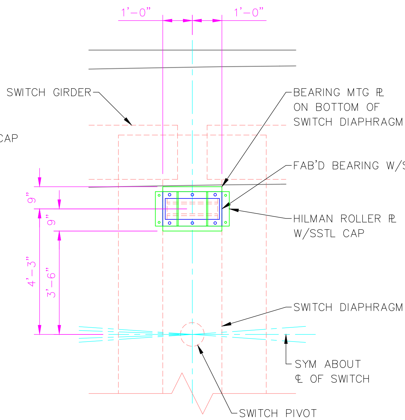
BEARING MOUNTING R. LOCATION PIER NO 5 SWITCH PIVOT
