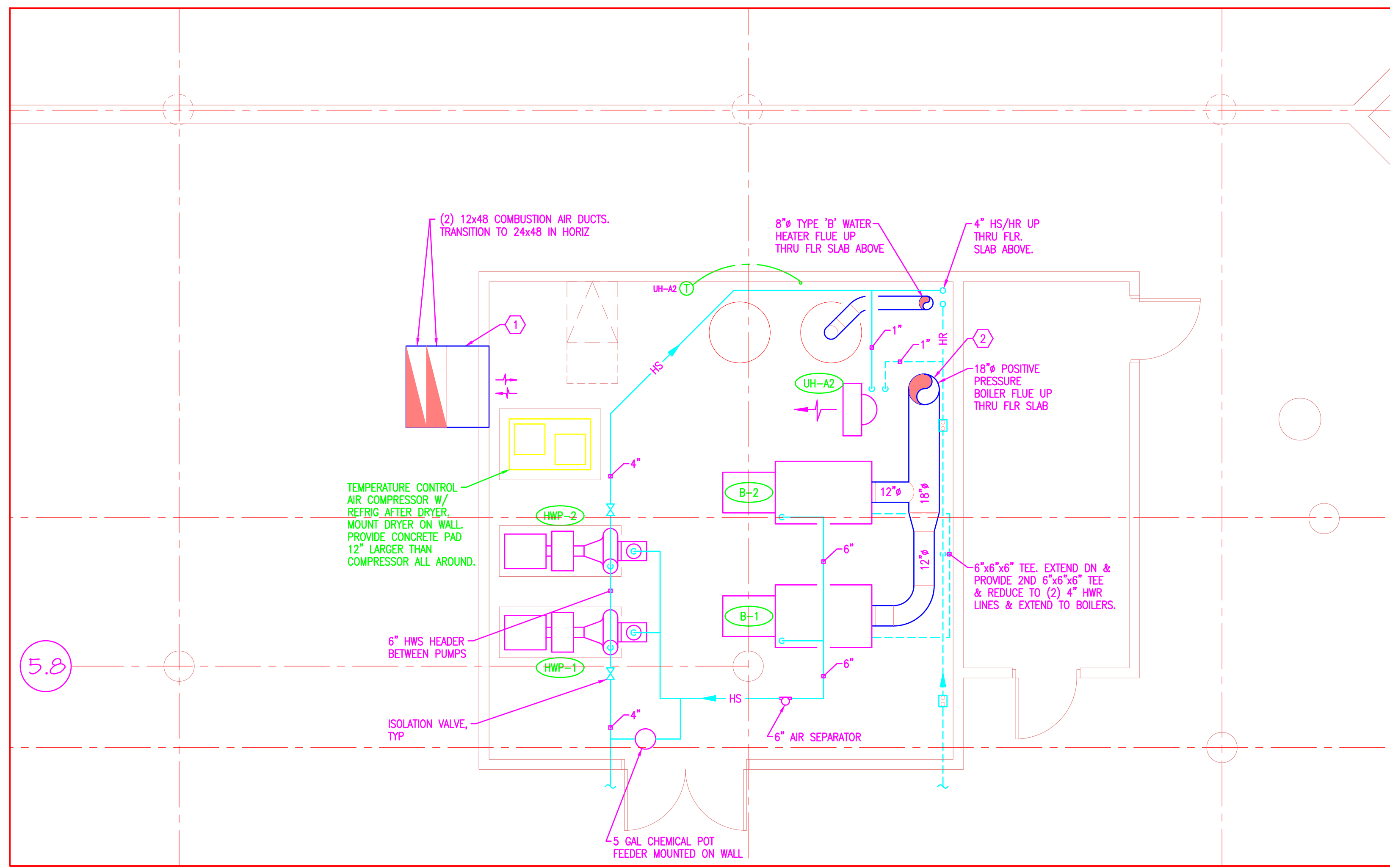
BOILER ROOM MECHANICAL PLAN SCALE: 1/4"=1'-0"
