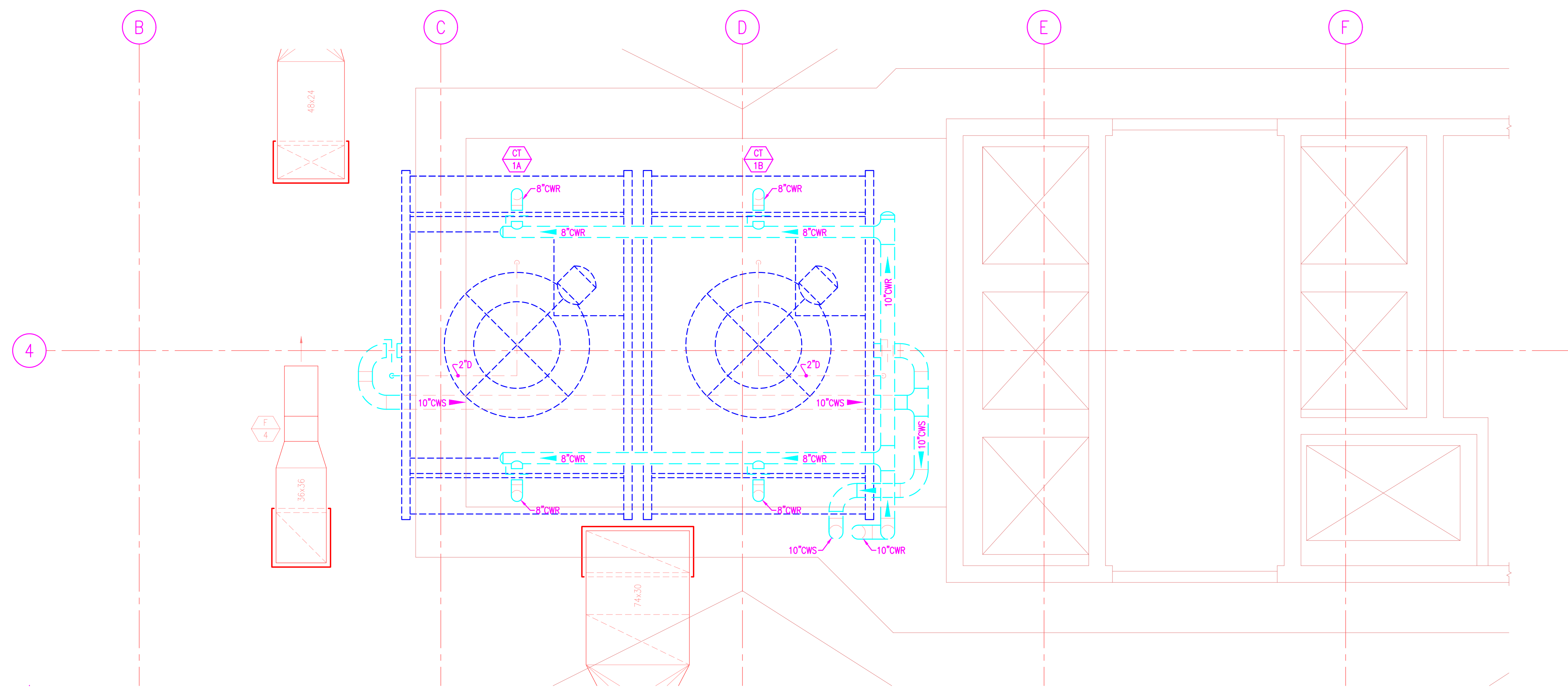
PARTIAL ROOF MECHANICAL DEMOLITION PLAN SCALE: 1/4"=1'-0"
