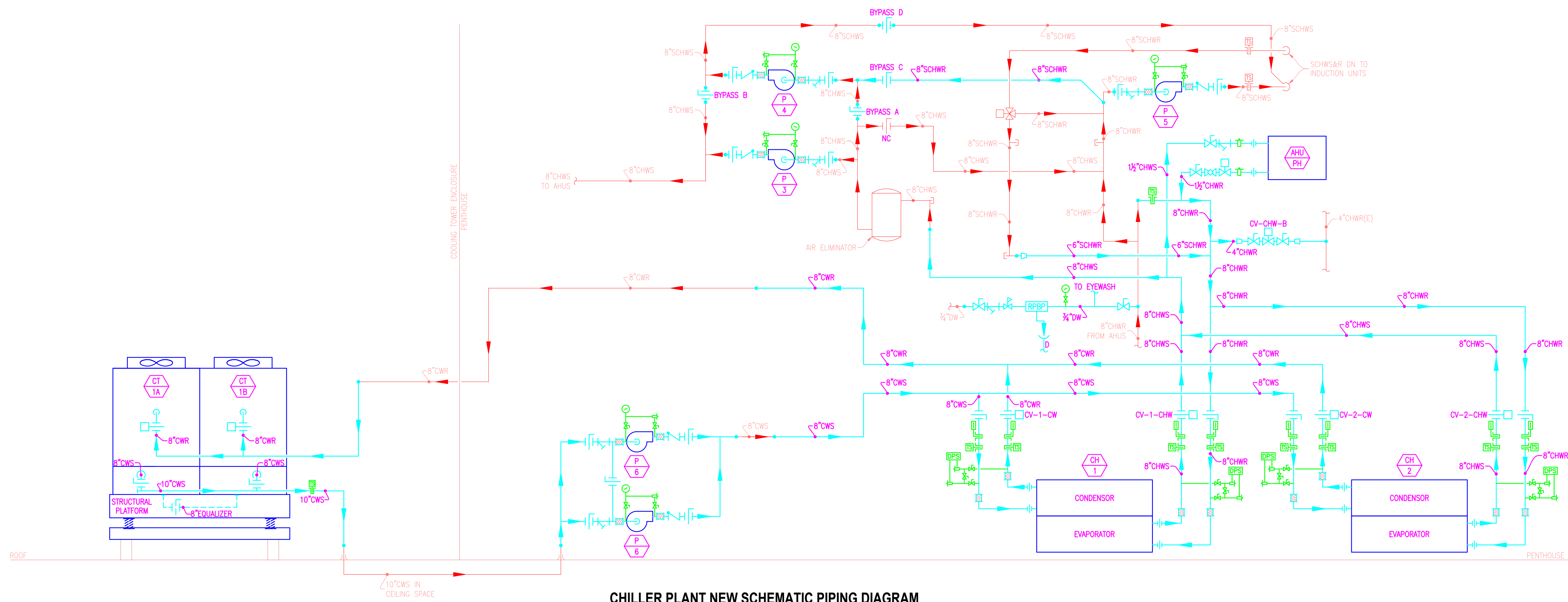
CHILLER PLANT NEW SCHEMATIC PIPING DIAGRAM NONE
