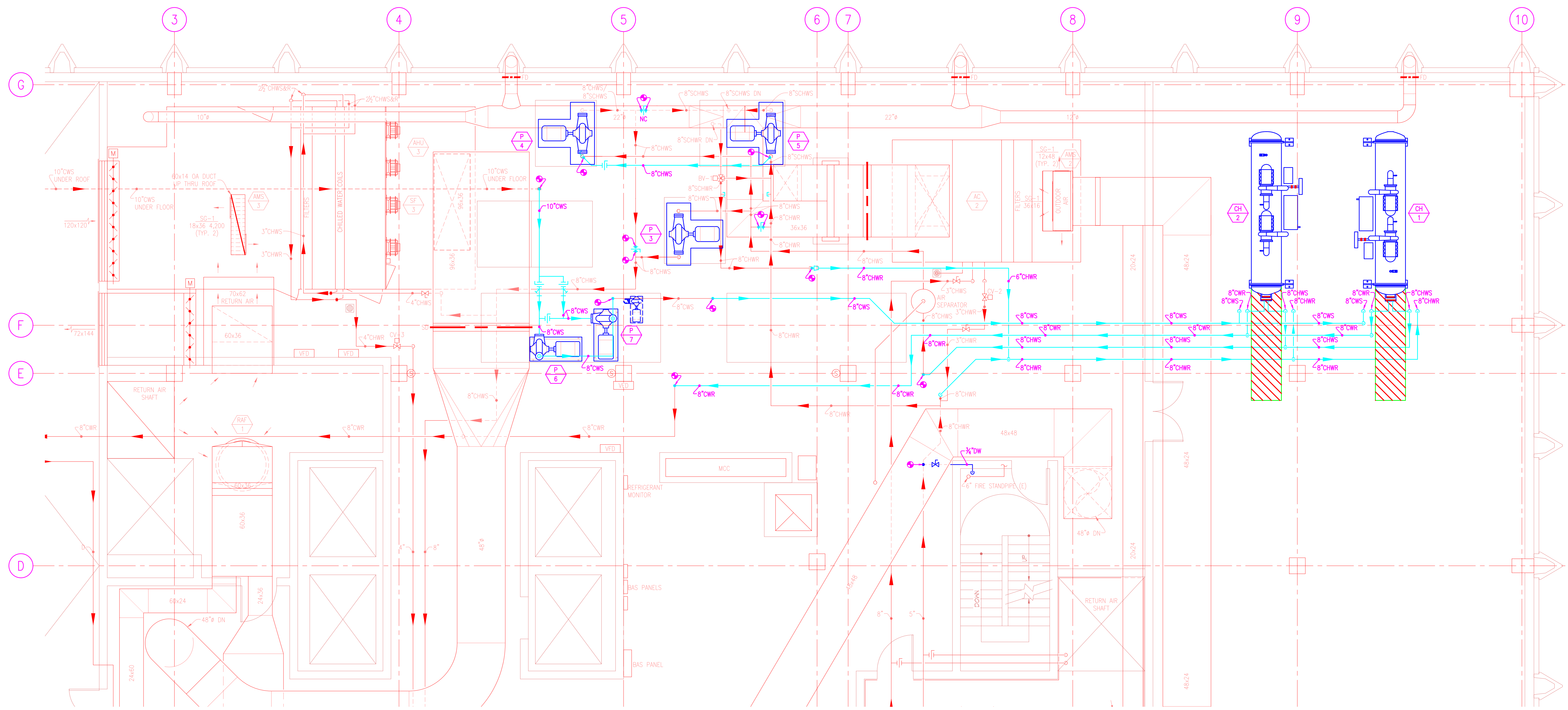
PENTHOUSE PARTIAL NEW MECHANICAL PLAN SCALE: 1/4"=1'-0"
