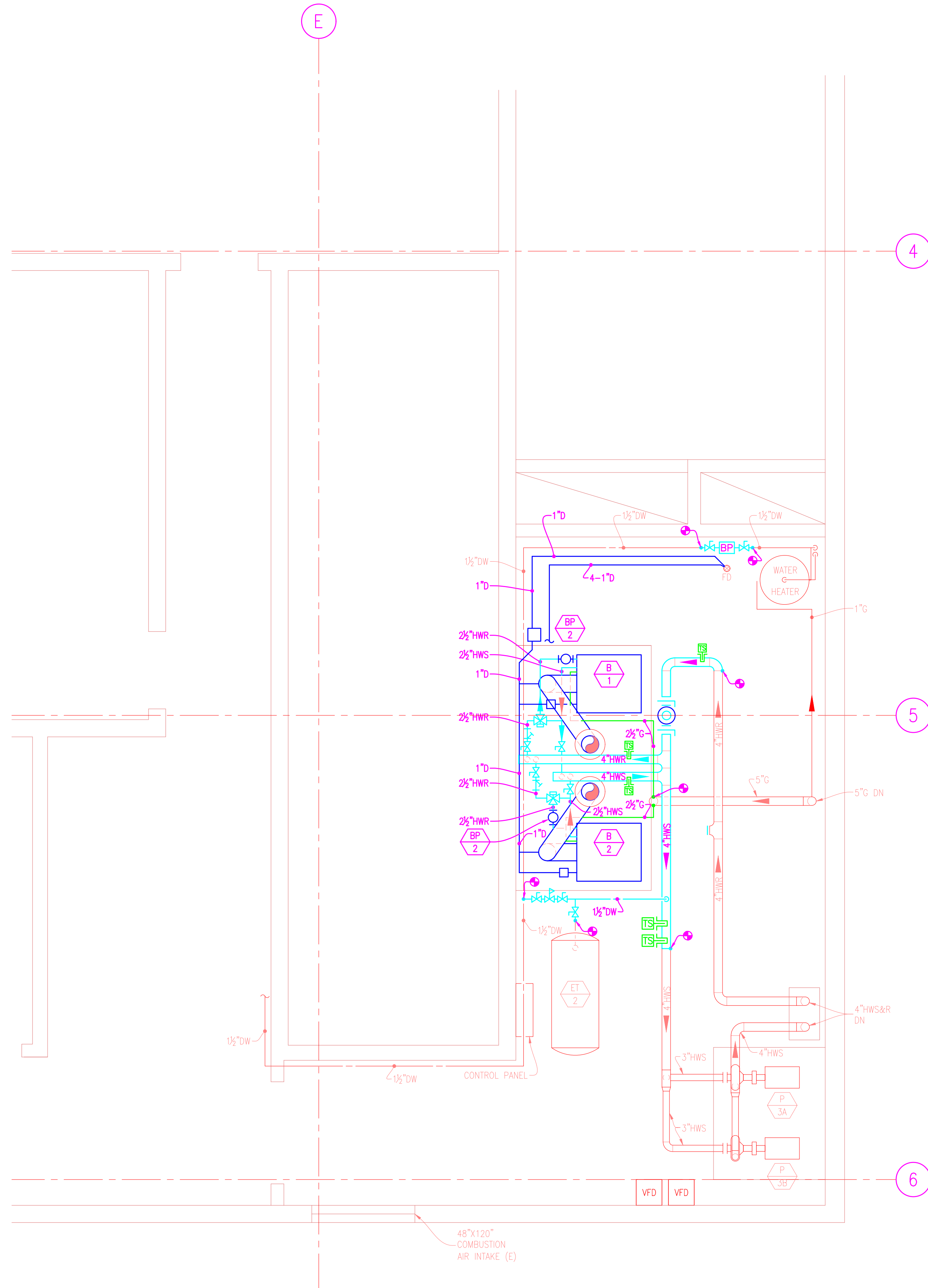
PARTIAL PENTHOUSE BOILER ROOM NEW MECHANICAL PLAN SCALE: 3/8"=1'-0"
