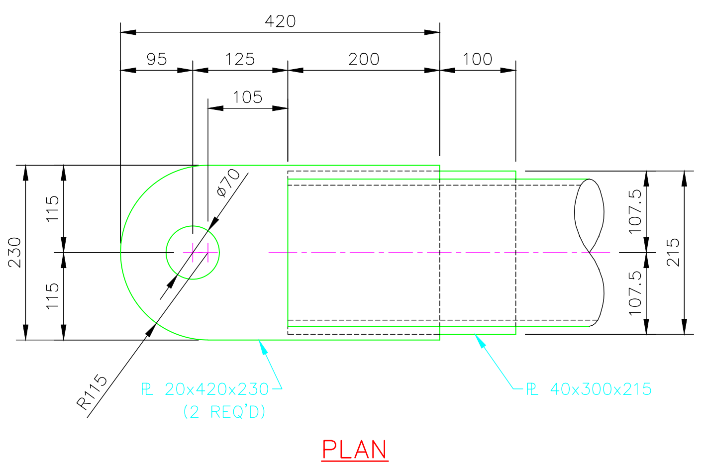
CLEVIS DETAIL
