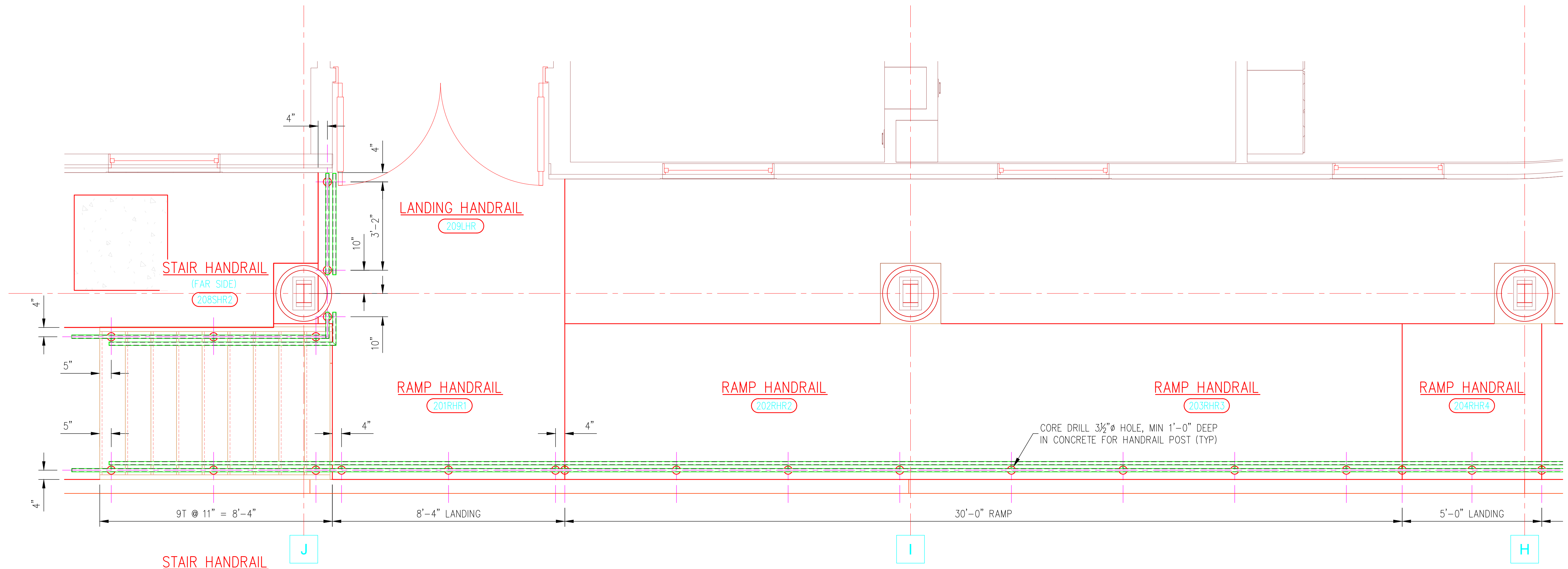
EXTERIOR RAMP HANDRAIL PLAN-SOUTH SCALE: 1/2"=1'-0"
