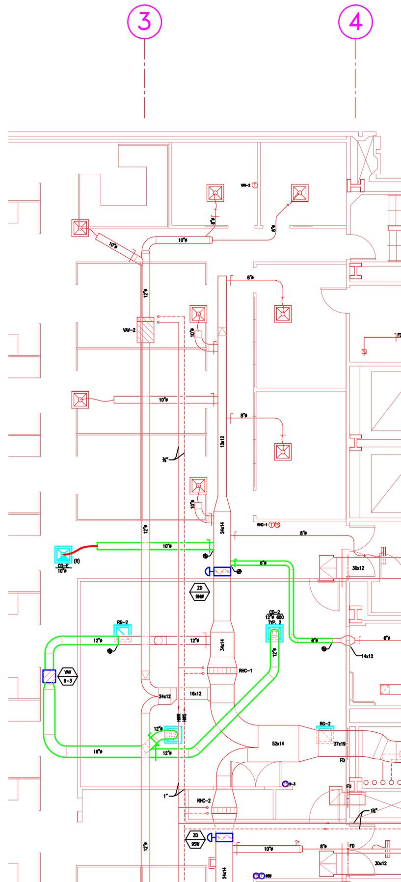
9TH FLOOR NEW MECHANICAL PLAN SCALE: 1/4"=1'-0"
