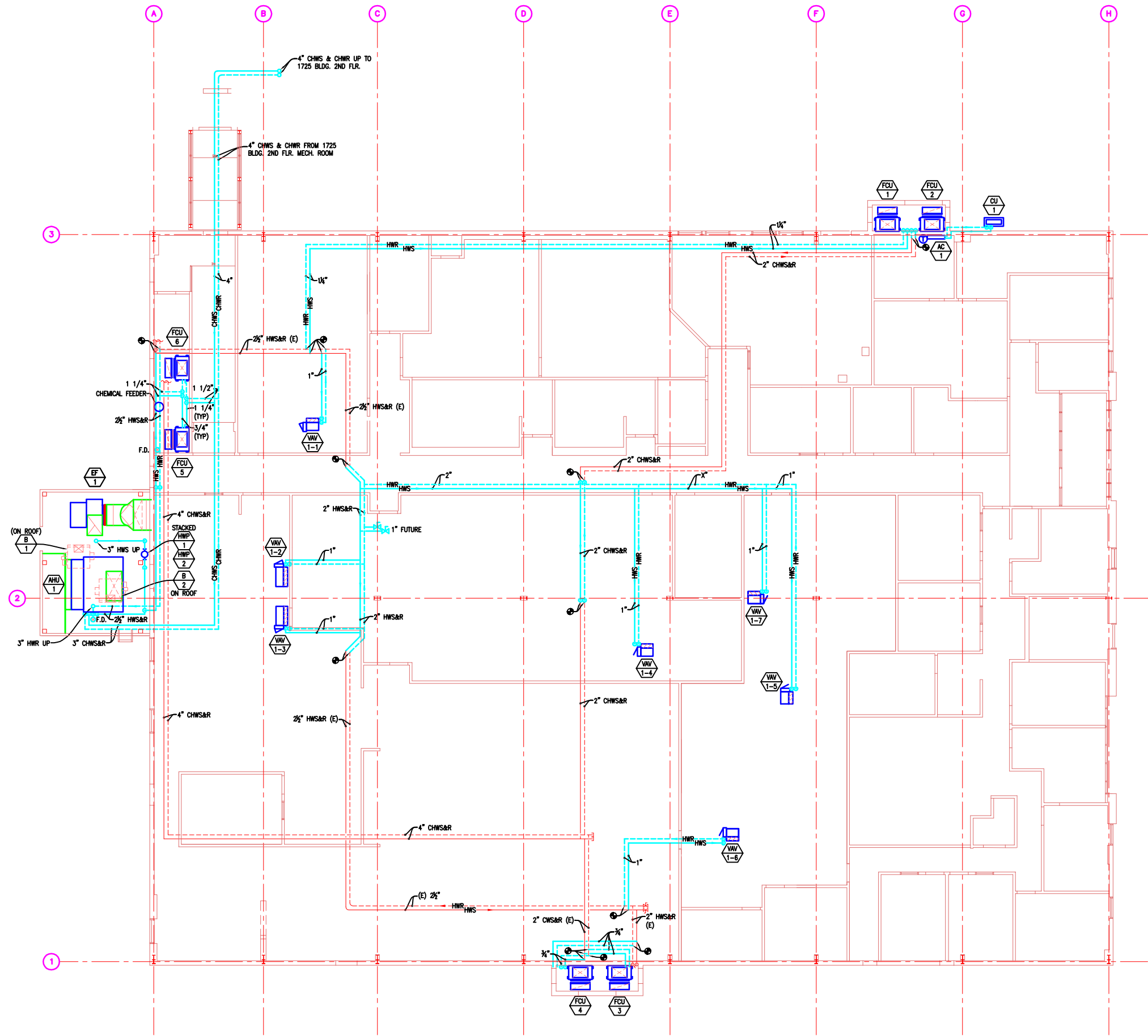
NEW MECHANICAL PIPING PLAN SCALE: 1/8"=1'-0"
