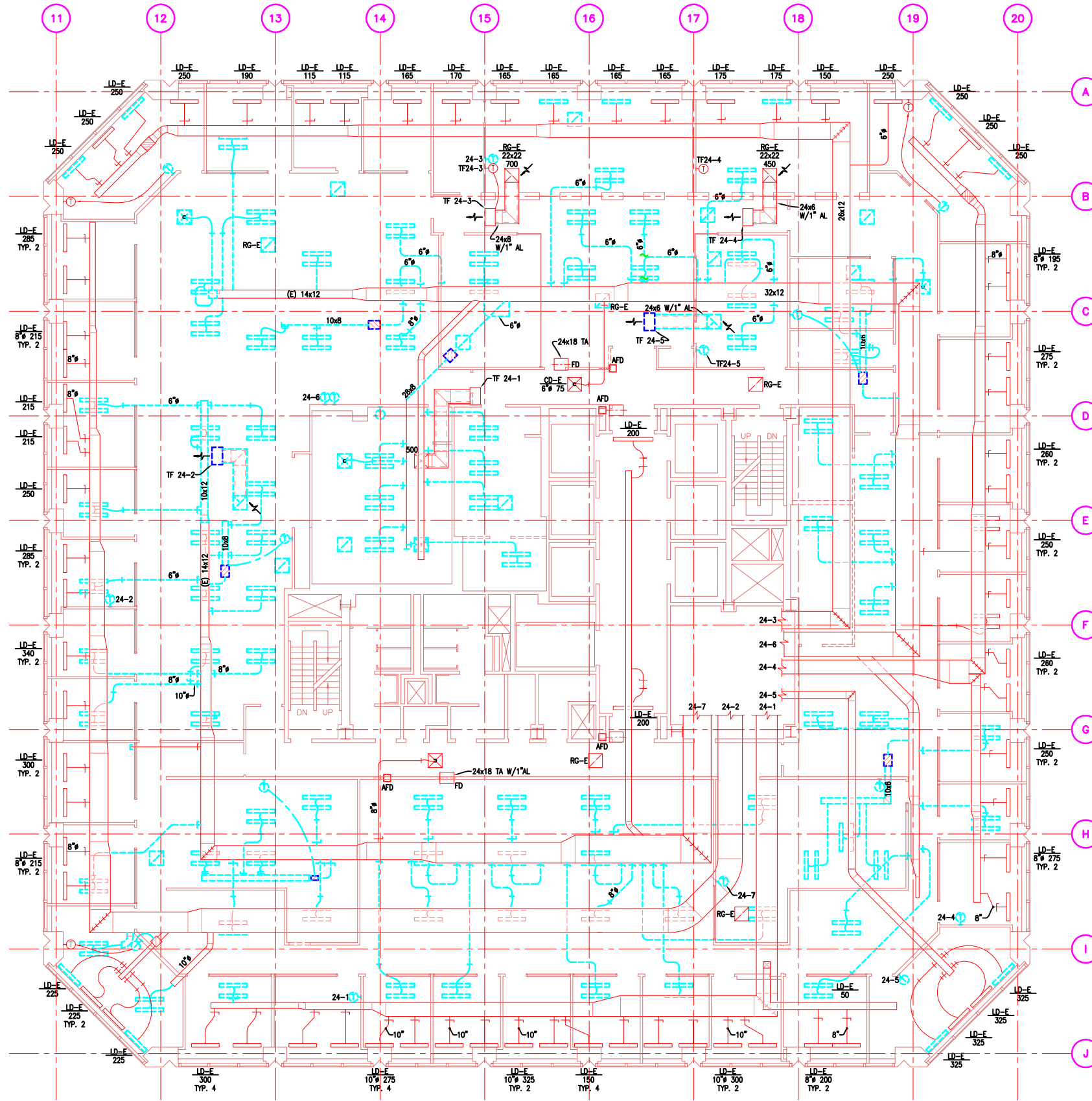
24TH FLOOR MECHANICAL DEMOLITION PLAN SCALE: 1/8"=1'-0"
