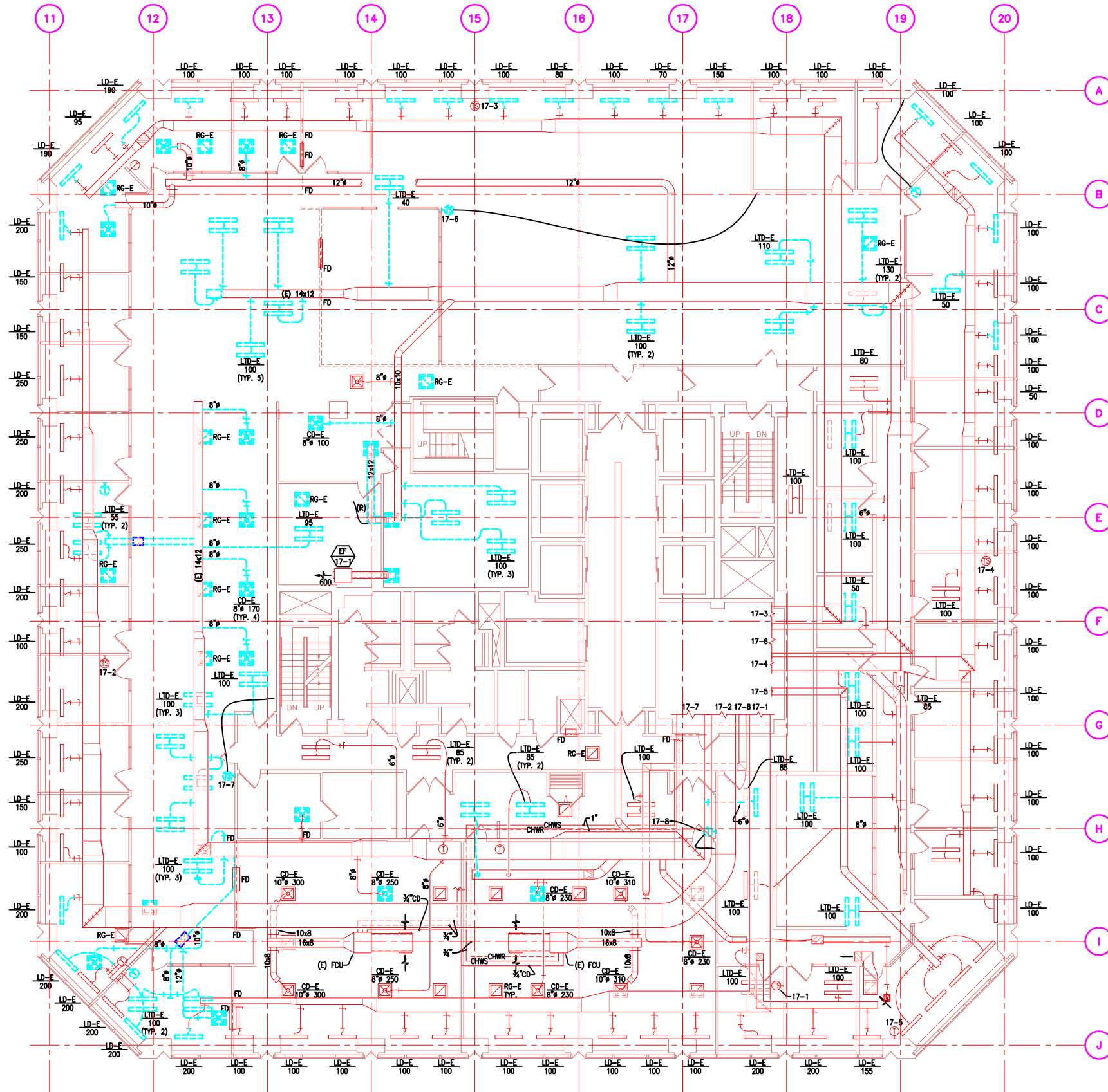
17TH FLOOR MECHANICAL DEMOLITION PLAN SCALE: 1/8"=1'-0"
