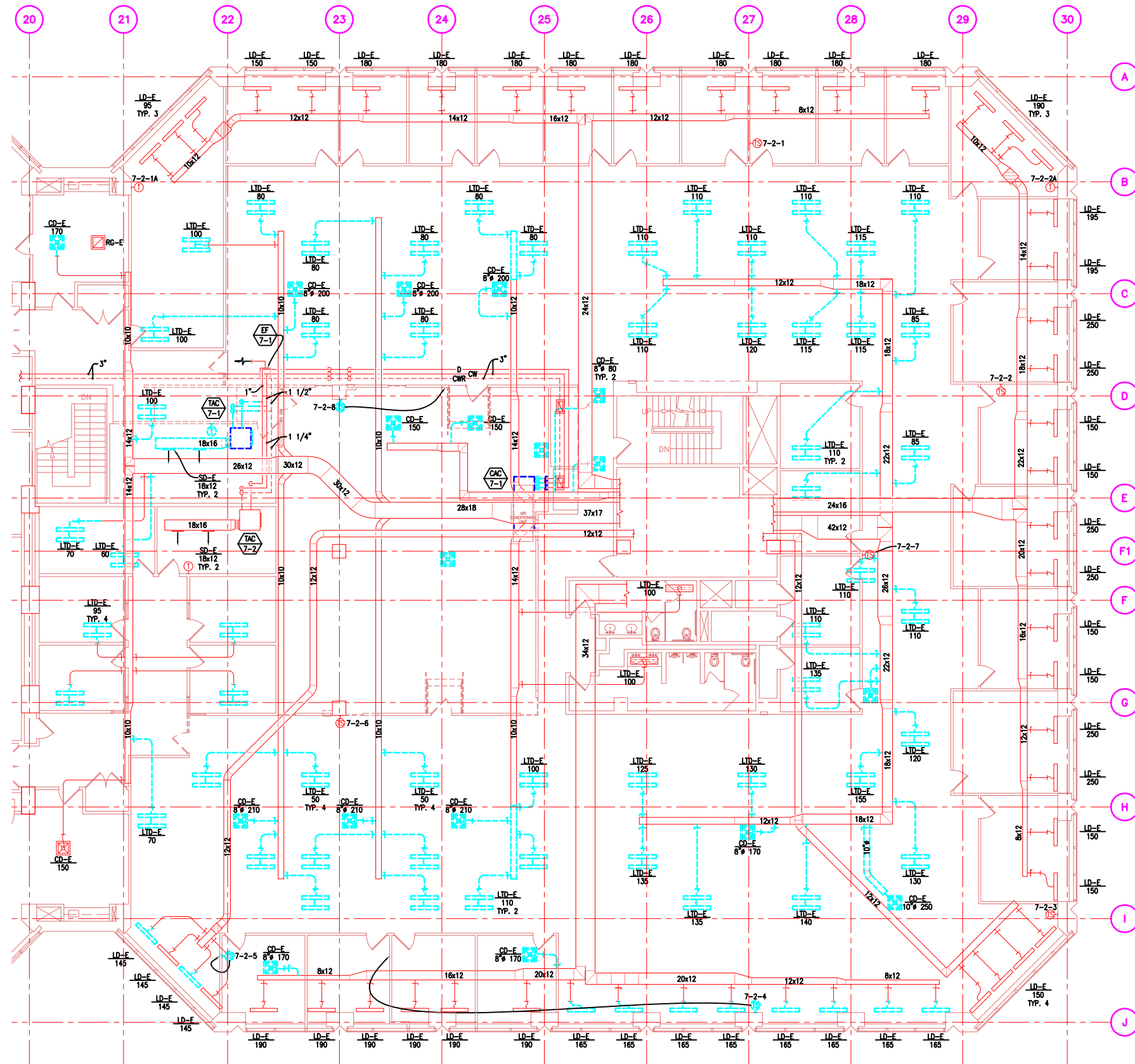
7TH FLOOR MECHANICAL DEMOLITION PLAN SCALE: 1/8"=1'-0"
