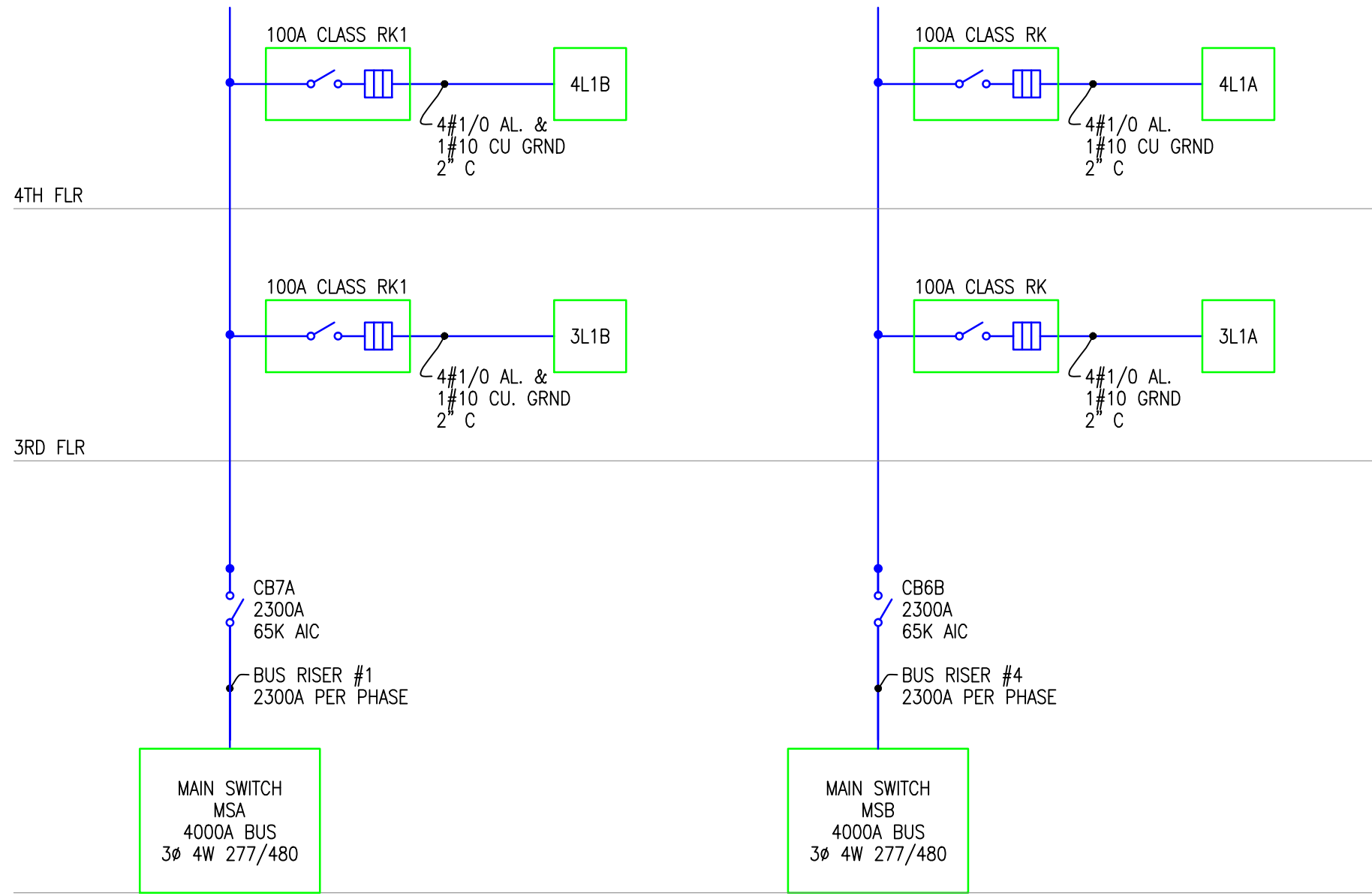
SINGLE LINE RISER DIAGRAM NO SCALE
