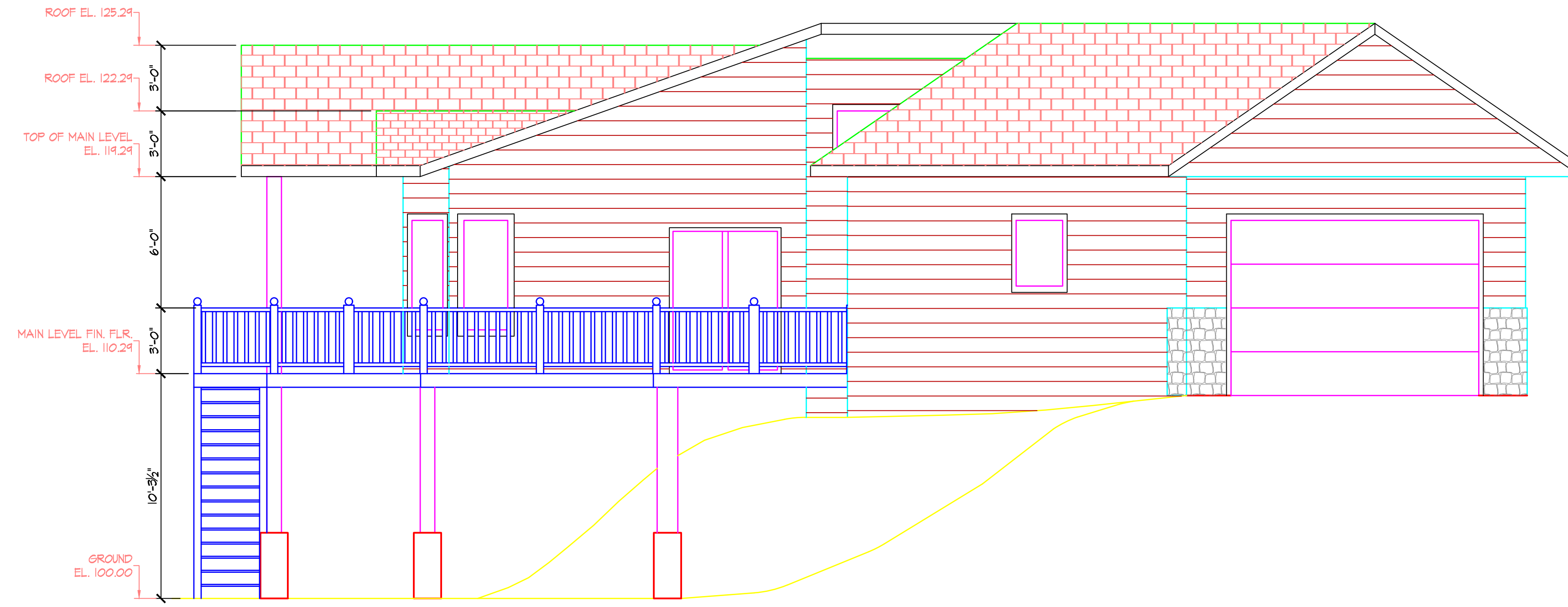
LEFT ELEVATION-LOOKING SOUTH SCALE: 1/4"=1'-0"
