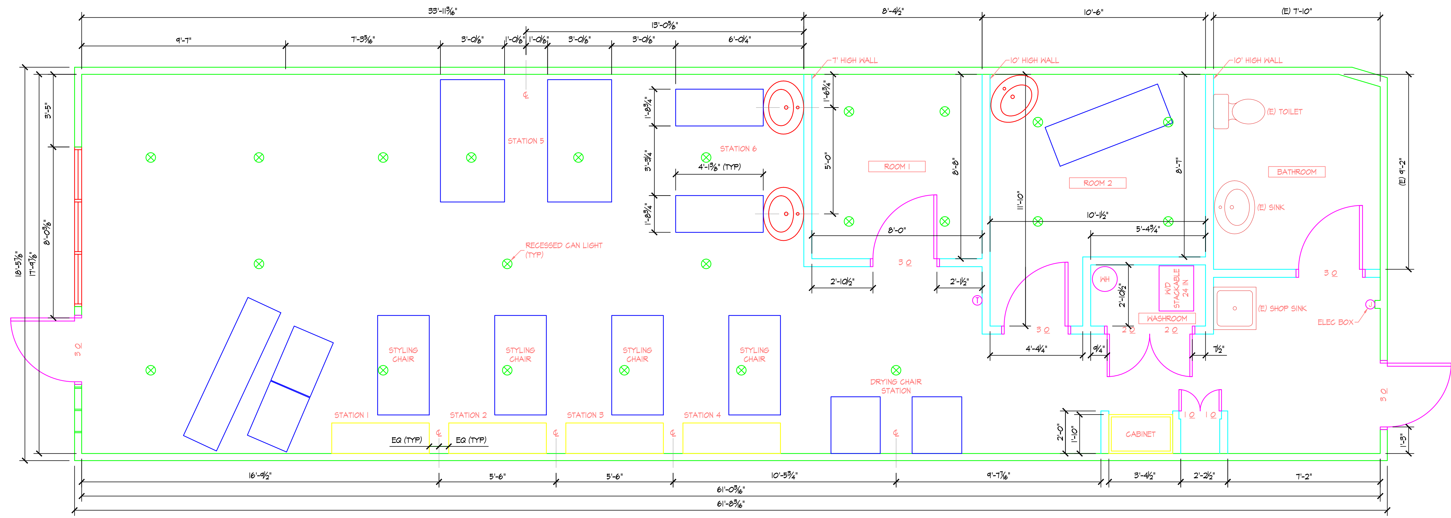
FLOOR PLAN SCALE: 3/8"=1'-0"
